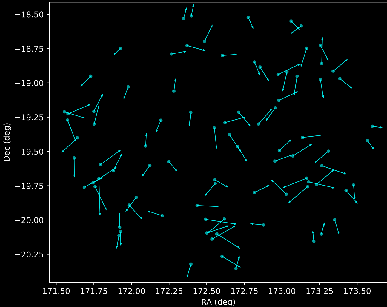
GALAH DR4 Noise Stream Proper Motion Vectors (n=87)
