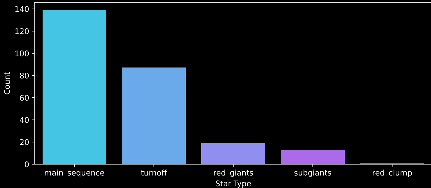
GALAH DR4 Field: [567] Count plot of Star Type
