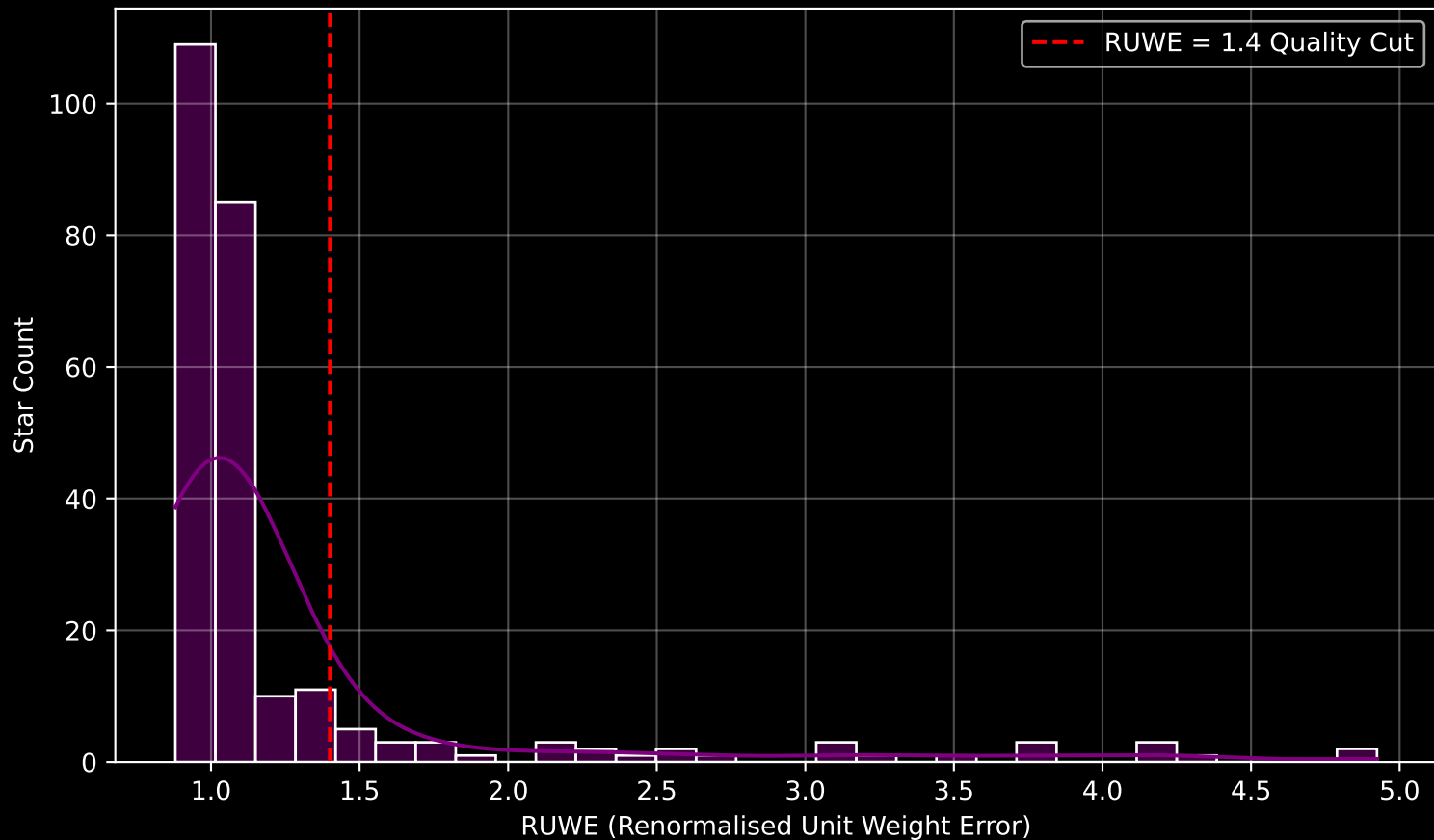
GALAH DR4 Field [567] RUWE Distribution (n= 250)
